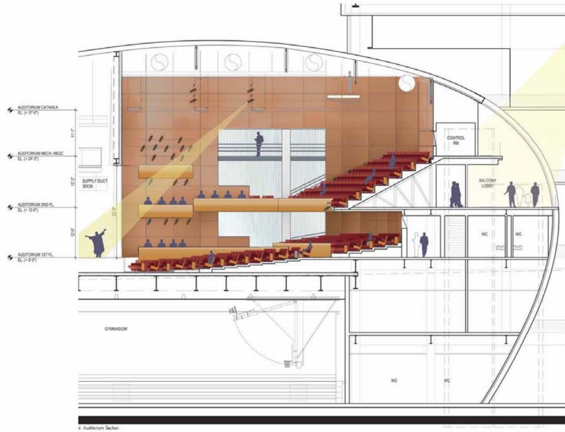
6 Auditorium Section
